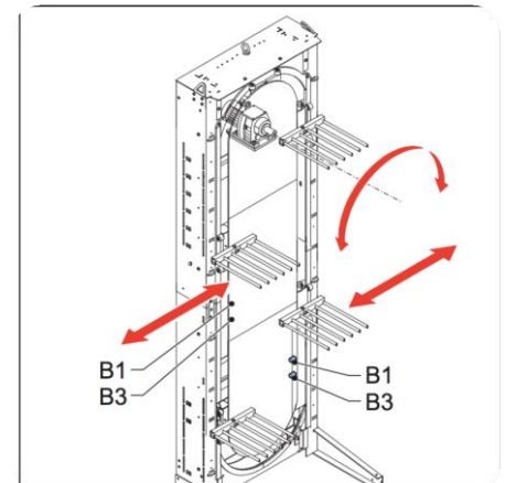
Fig. 3 Descending / Ascending carrier
